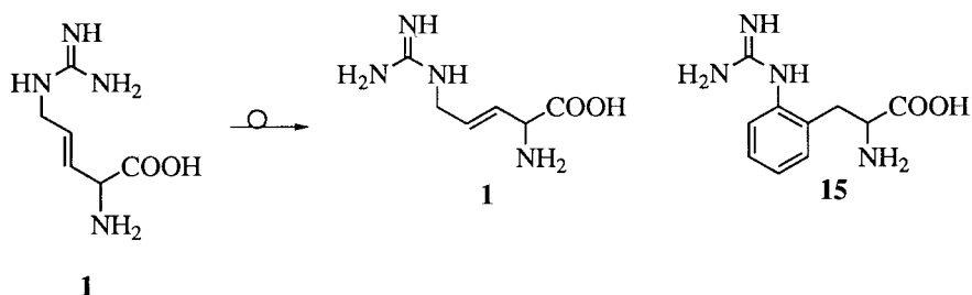
Figure 1. Comparison of specific conformations of 1 and 15 .
