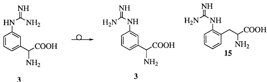
Figure 2. Comparison of specific conformations of 3 and 15 .
